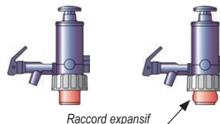
Raccord expansif
